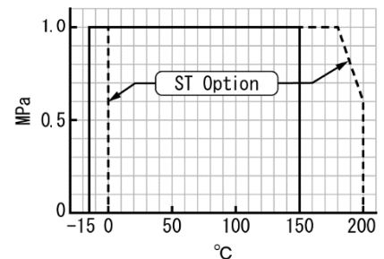
Pressure & Temperature rating (100 to 150A)
