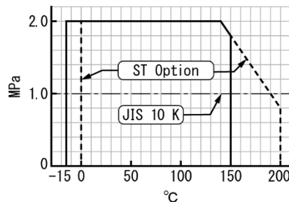
Pressure & Temperature rating (25 to 80A)
