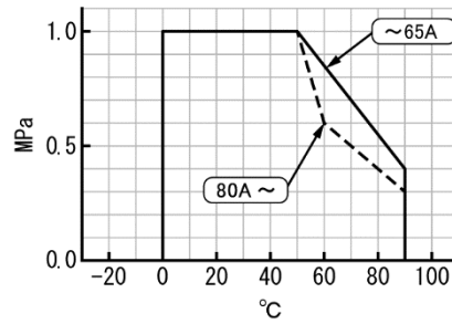
| Pressure & Temperature rating (C-PVC)
