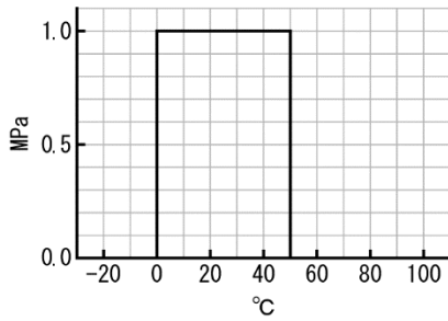
| Pressure & Temperature rating (PVC)
