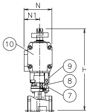
TADBS901TTF-015 TADBS901TTF-020
