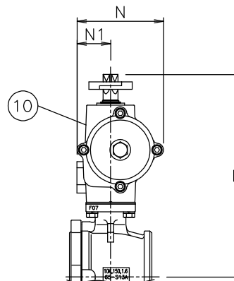
TADBS9*1TTF-065 TADBS9*1TTF-080
